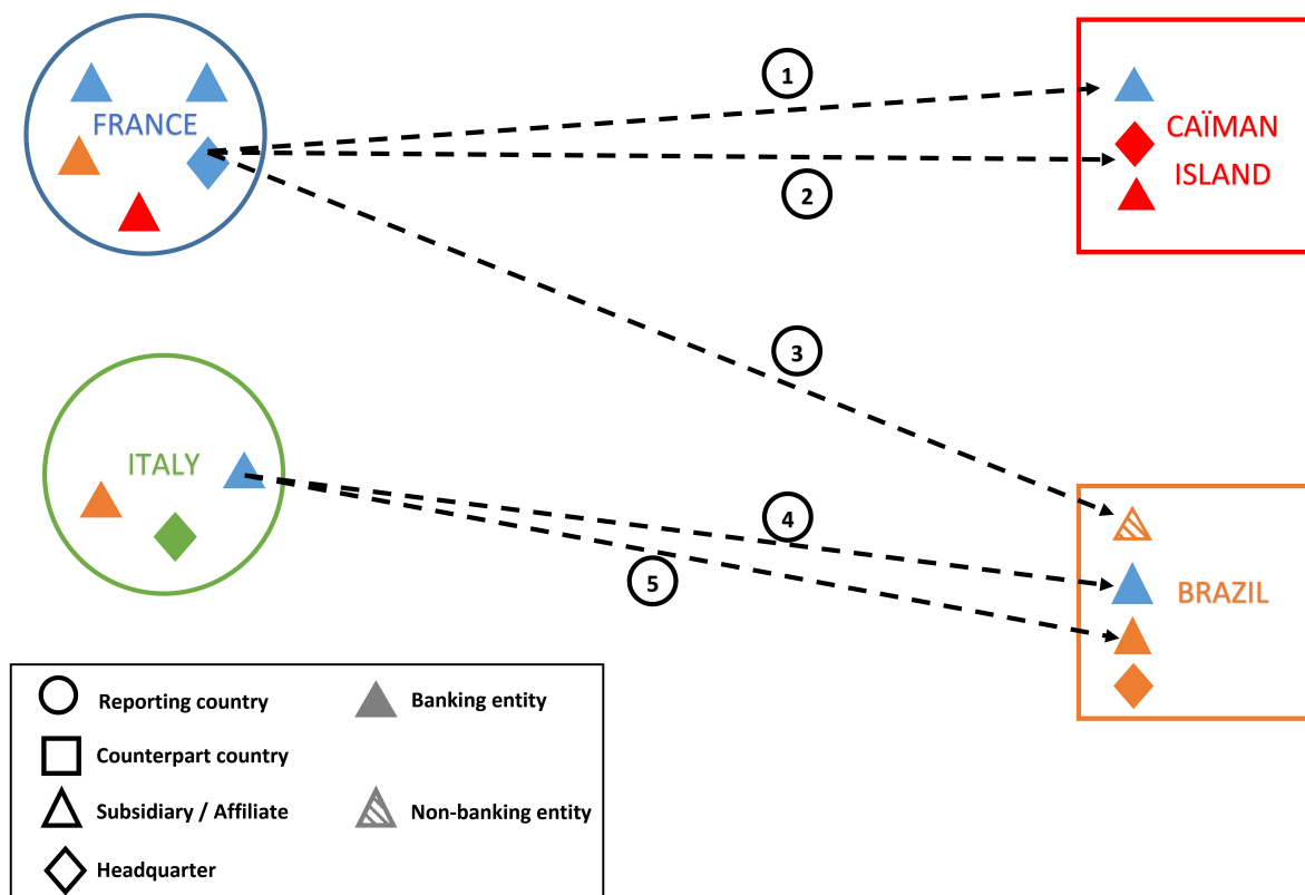
Figure 9: Structure of the LBSN dataset
